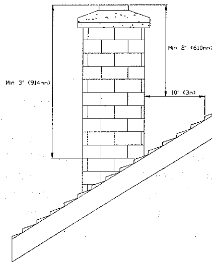
FIGURE 2.2 Minimum Height of the Chimney
