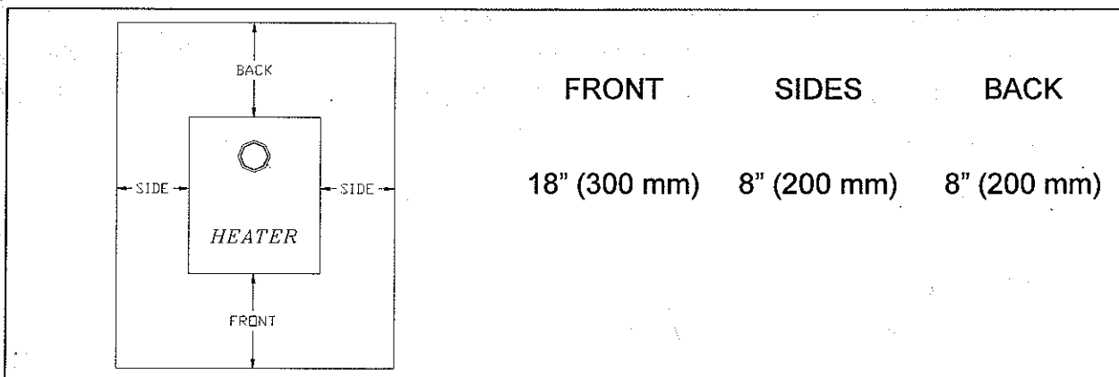
FIGURE 1.4 Floor protector
