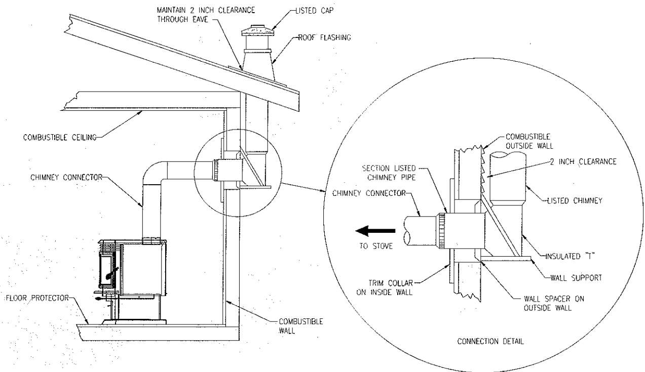
FIGURE 2.2.1 (A) Typical installation through the wall
